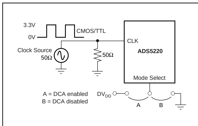
FIGURE 6. General Input Clock Interface of ADS5220.
